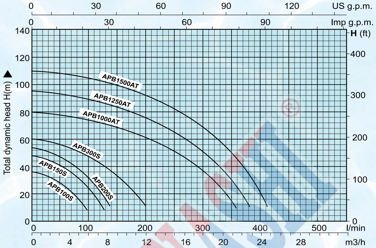
PERFORMANCE CURVE AT 2900 R.P.M.
